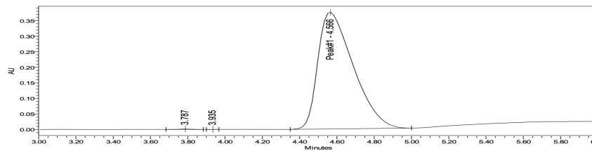
HPLC-UV Chromatogram
