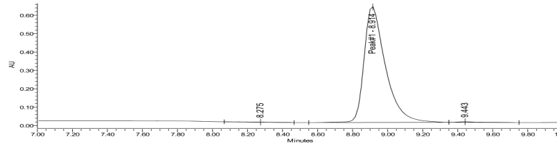
HPLC-UV Chromatogram
